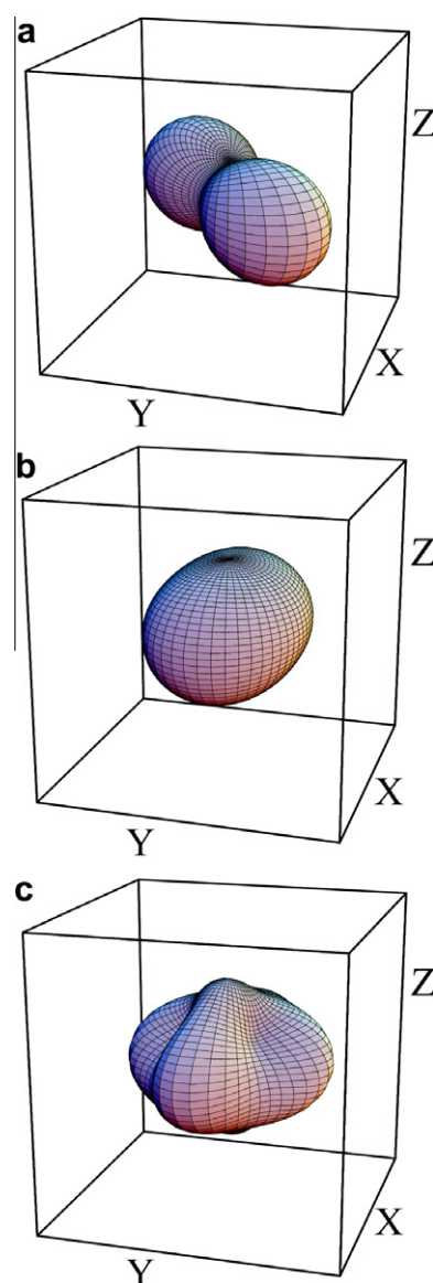
Fig. 9. Orientation distribution functions for probe R1 in cis -form: (a) at 77 K, determined within OD approach; (b) at 295 K, determined within OP approach with expansion rank 2; (c) at 295 K, determined within OP approach with expansion rank 4.
