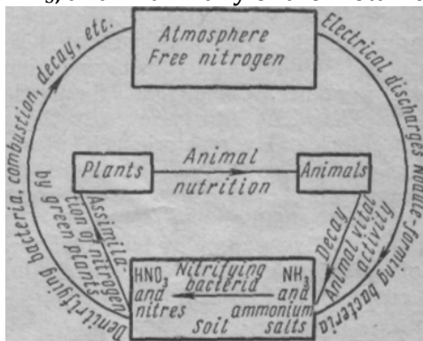
Fig. 1 Nitrogen cycle in nature
